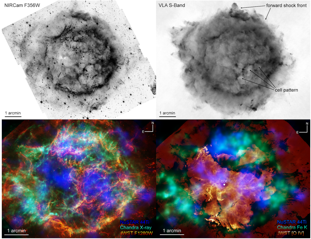
Figure 3.21: Multiwavelength views of the young Galactic supernova remnant Cassiopeia A [75]. The upper panels compare the JWST/NIRCcam F356W image with a VLA S-band radio image. The lower left panel combines the NuSTAR ^{44}\text{Ti} map, the Chandra 1 Msec X-ray image, and the JWST/MIRI F1280W image, while the lower right panel combines the JWST unshocked ejecta 25.89\,\mu\text{m} line map, the NuSTAR ^{44}\text{Ti} map, and the Chandra Fe-K map. The radio and X-ray emission trace nonthermal synchrotron radiation and shock-heated material, whereas the infrared emission probes dust and ejecta/CSM structures. The radioactive isotope ^{44}\text{Ti} traces material synthesized in the innermost ejecta and provides a late-time diagnostic of asymmetric nucleosynthesis and explosion dynamics. The black circle marks the location of the central neutron star, while the white circle marks the location of the center of expansion (COE).
