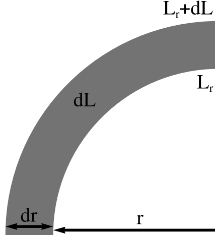
Figure 2.4: Luminosity through a spherical shell.
