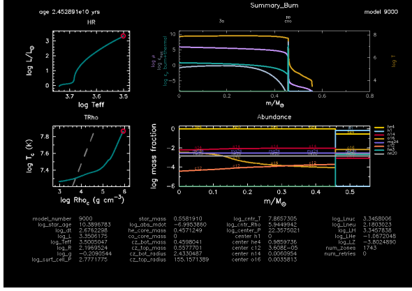
Figure 1.10: Stellar profiles before the first helium flash for 0.8M_{\odot} star based on MESA test suite 1M_pre_ms_to_wd [11]. In the outer regions of the star, H-shell burning is ongoing. The maximum temperature is located off-center.
