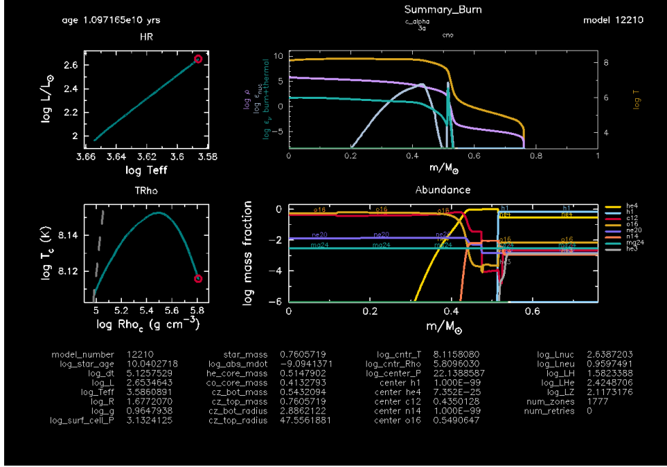
Figure 1.14: Stellar profiles around the early-AGB for 1.0M_{\odot} star based on MESA test suite 1M_pre_ms_to_wd [11]. From \epsilon_{\text{nuc}} , one can identify the shell where helium fusion occurs, the shell where hydrogen fusion occurs, and the inter-shell region between them.
